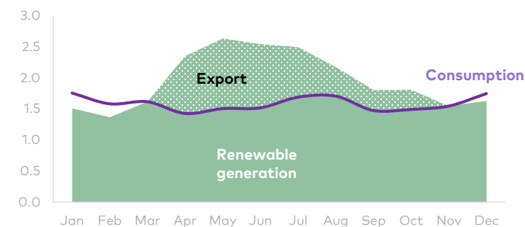
Generation, baseline scenario 2035
