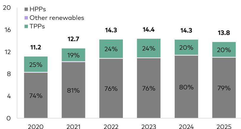
Figure 1: Electricity generation, TWh
